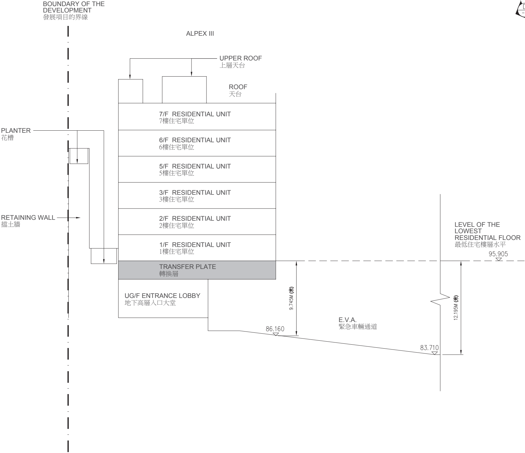
CROSS-SECTION D
