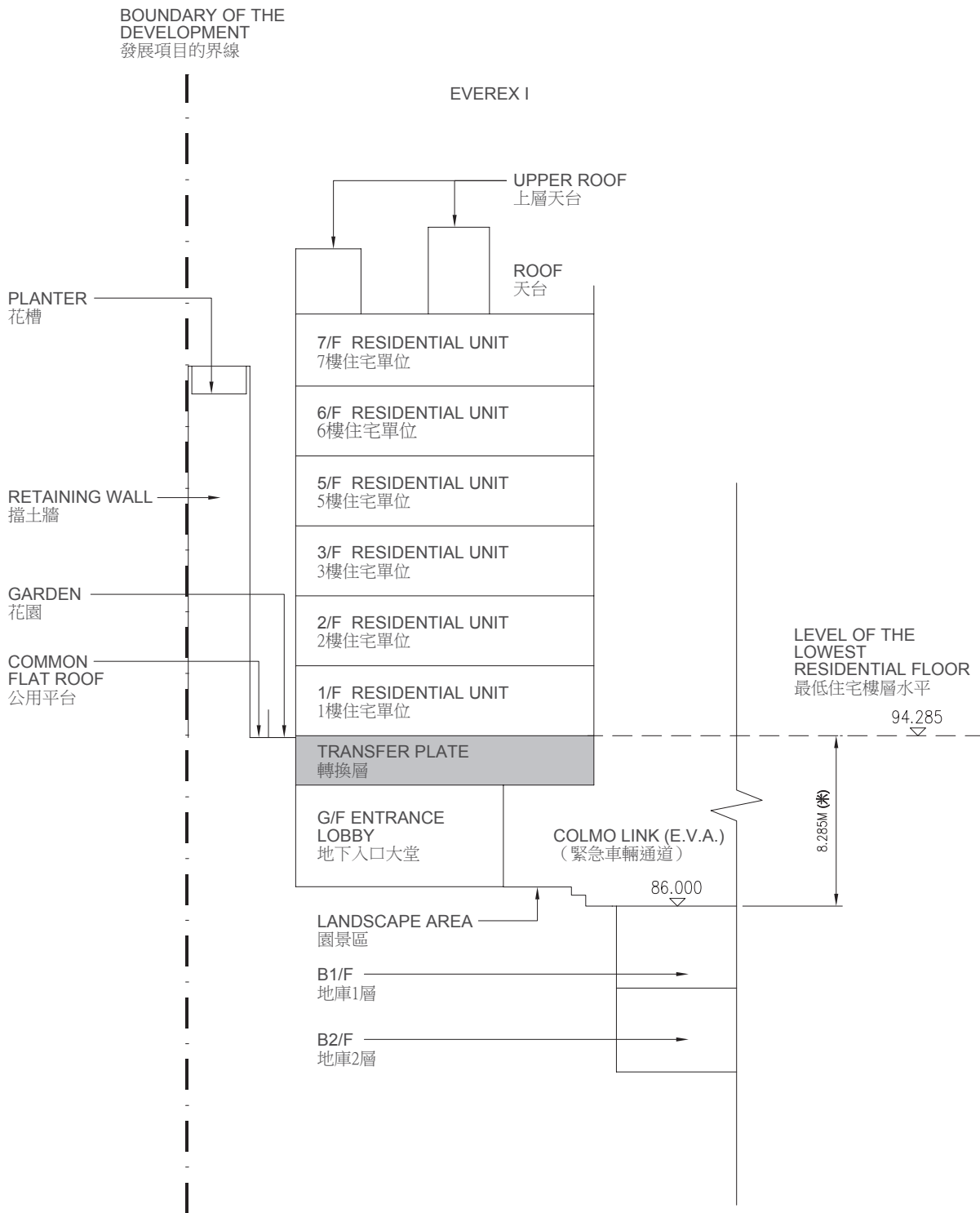
CROSS-SECTION F
